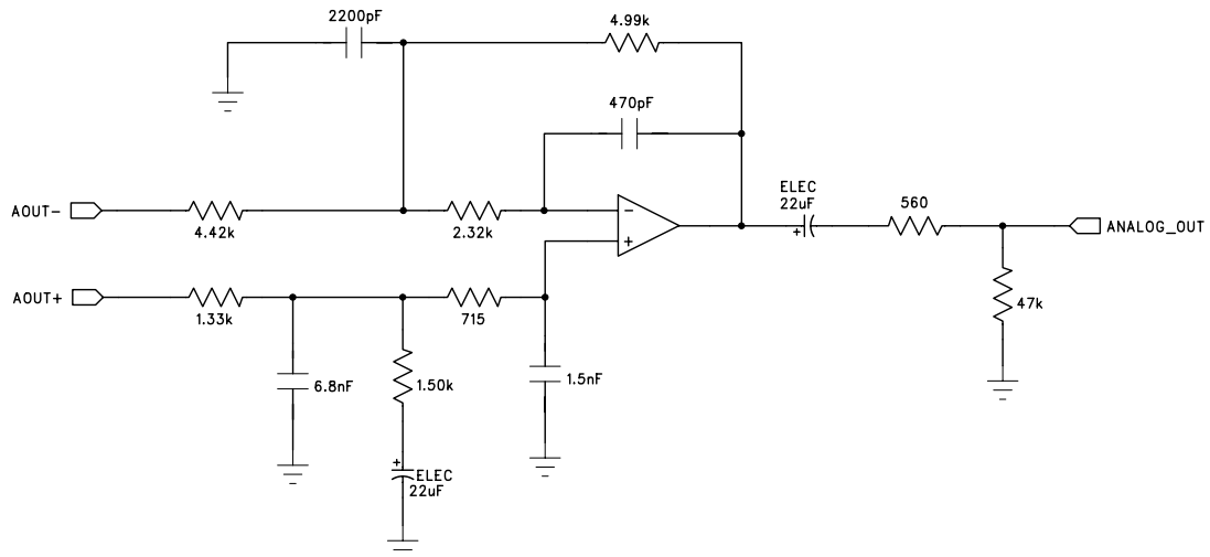
Figure 42. Recommended Output Filter
